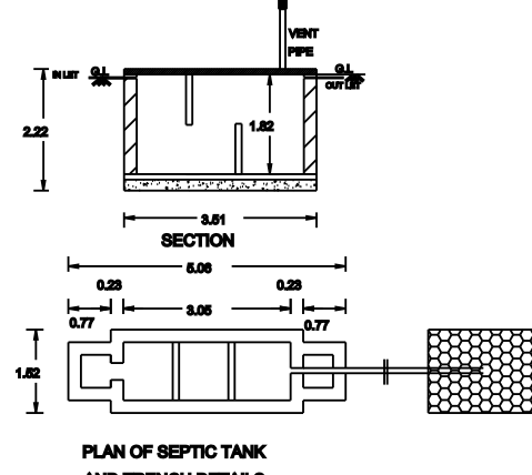
PLAN OF SEPTIC TANK AND TRENCH DETAILS
