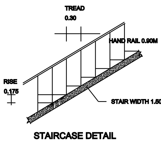
STAIRCASE DETAIL
