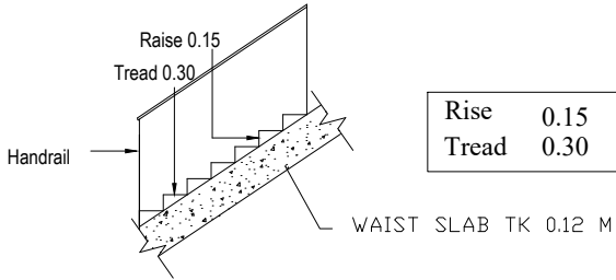
STAIRCASE DETAIL
