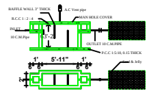
Septic tank and trench
