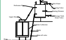
Details Of Solar Water Heater (NTS)
