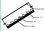
Stair
