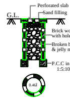
PERCOLATION PIT (NOT FOR SCALE)
