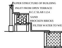
Rainwater harvesting
