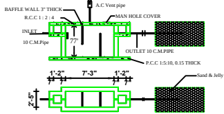
Septic tank and trench
