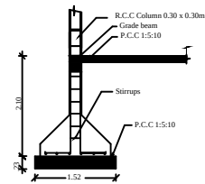
Column Detail
