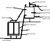
Details Of Solar Water Heater (NTS)
