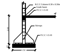
Column Detail
