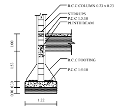
COLUMN DETAILS
