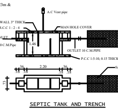
SEPTIC TANK AND TRENCH
