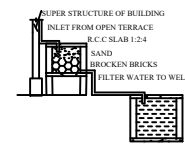
Rainwater harvesting
