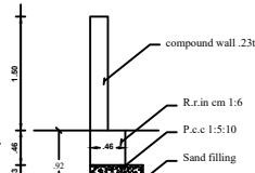
Compound Wall Detail
