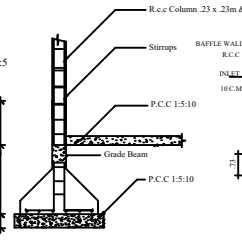
COLUMN DETAIL
