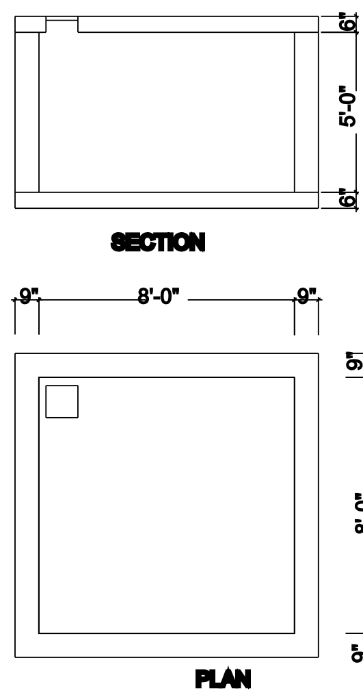
DETAILS OF COLLECTION GRUP FOR RAIN WATER HARVESTING OF ROOF TOP RAIN WATER.
