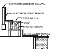
DETAILS OF FILTER BED & WELL NTS
