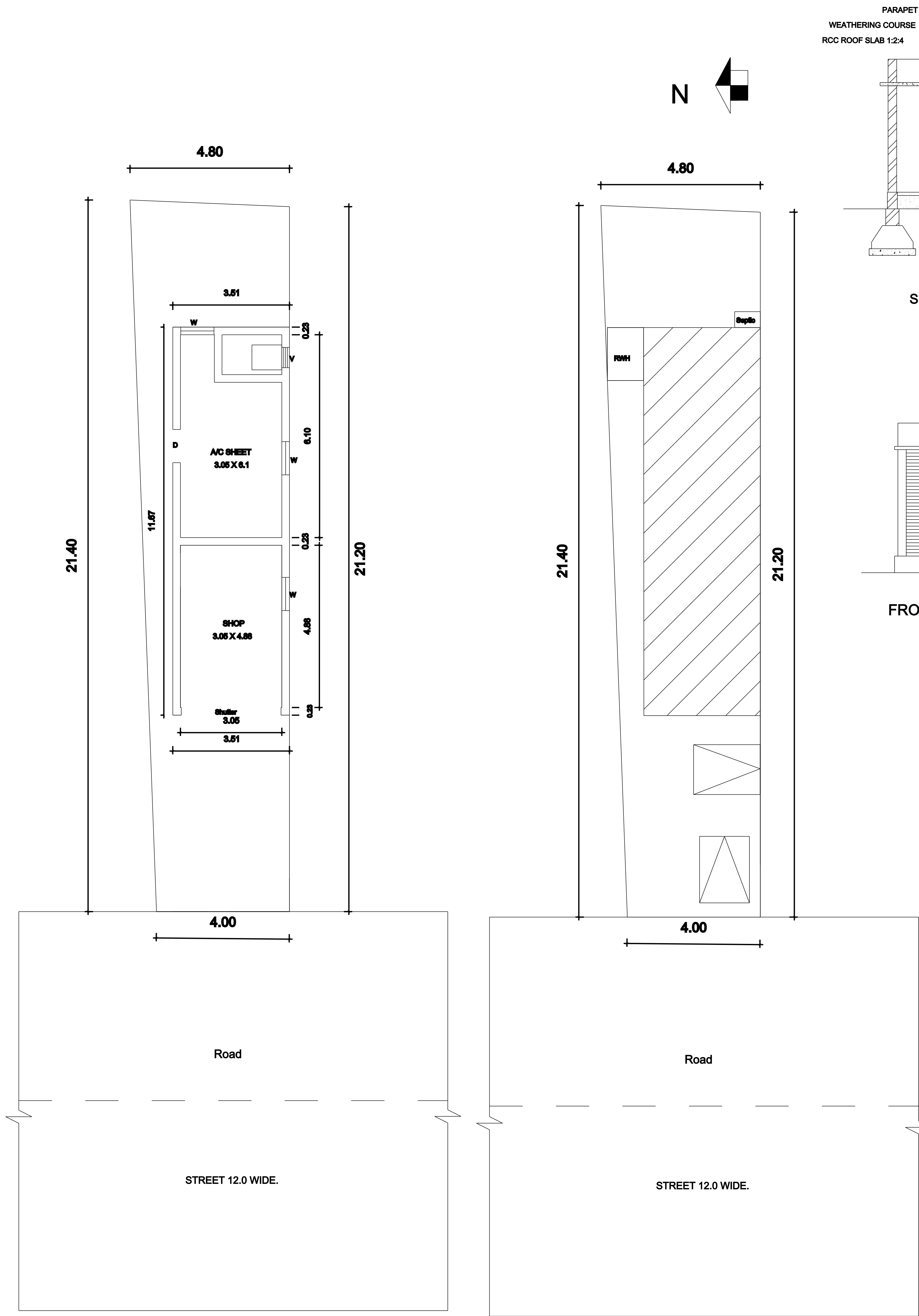
PRO. GROUND FLOOR PLAN.
