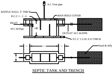
SEPTIC TANK AND TRENCH
