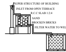
Rainwater harvesting
