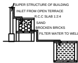
RAINWATER HARVESTING
