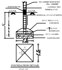
FOUNDATION DETAIL (SCALE: 1:30)
