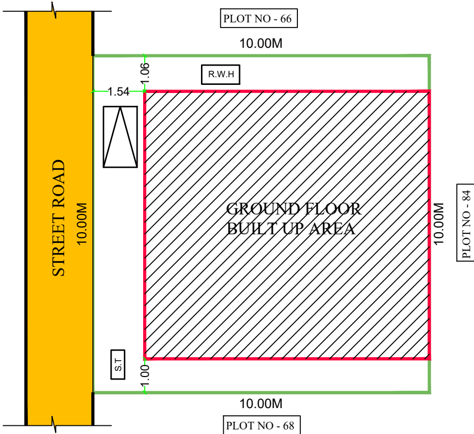
SITE PLAN
