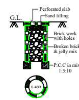
PERCOLATION PIT (NOT FOR SCALE)
