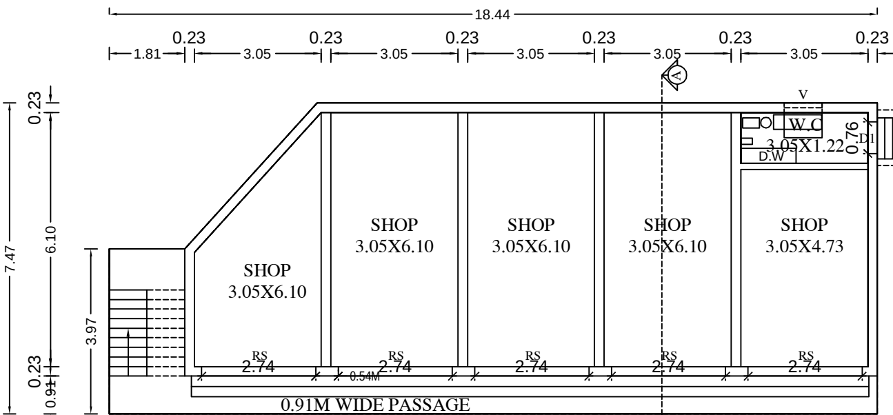
PRO. GROUND FLOOR PLAN
