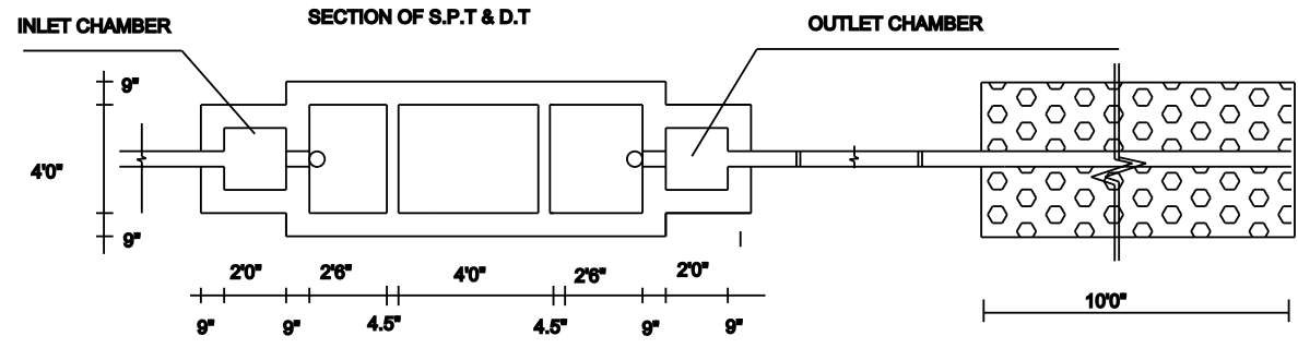
SEPTIC TANK DETAILS
