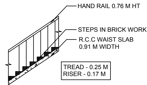
STEP DETAILS
