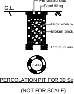
RAINWATER HARVEST
