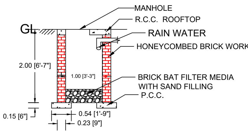
SECTION ON O - P
