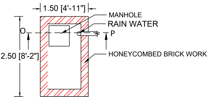
PLAN RAIN WATER HARVESTING
