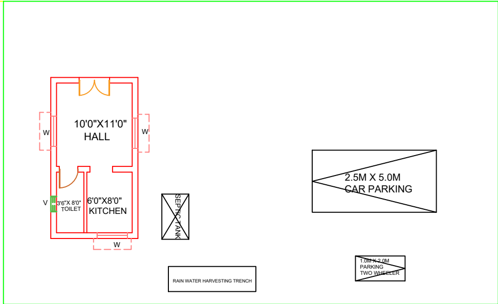
SITE PLAN
