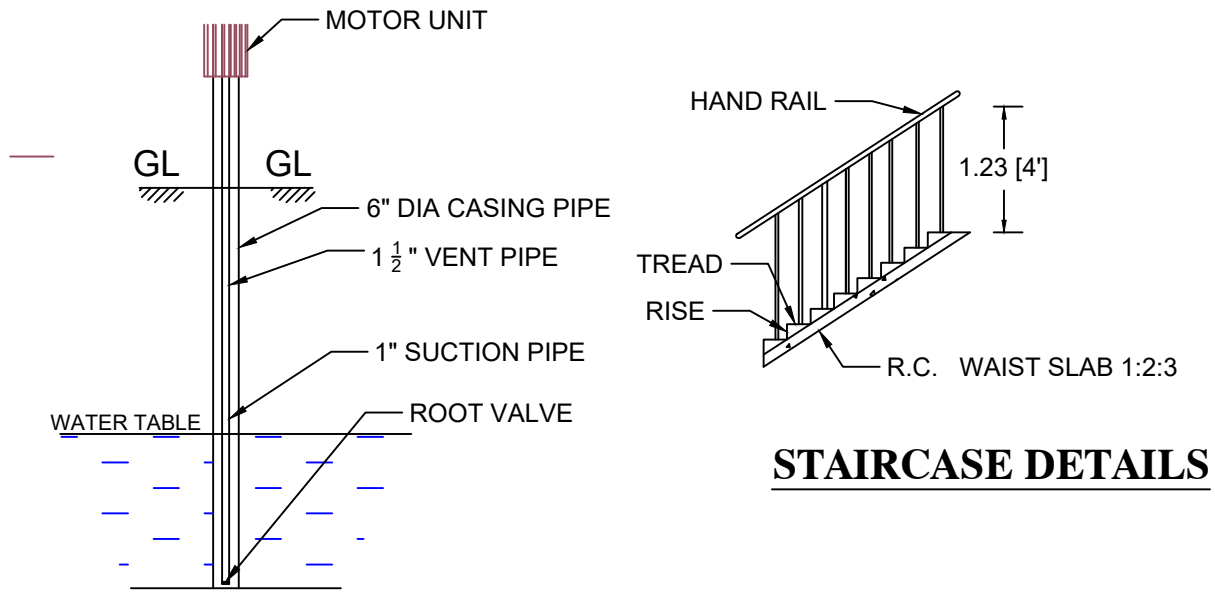
SEC.OF BOREWELL
