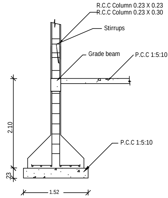
COLUMN DETAIL
