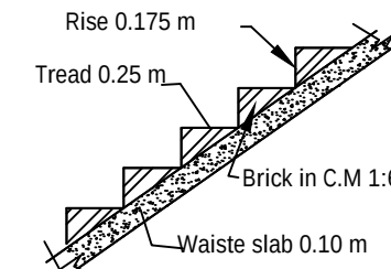
STAIR DETAILS
