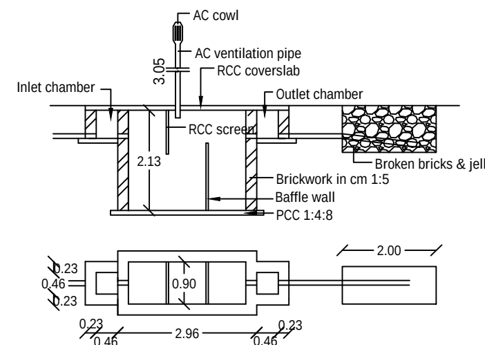
SEPTICTANK DETAILS
