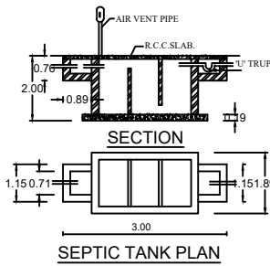
SEPTIC TANK PLAN
