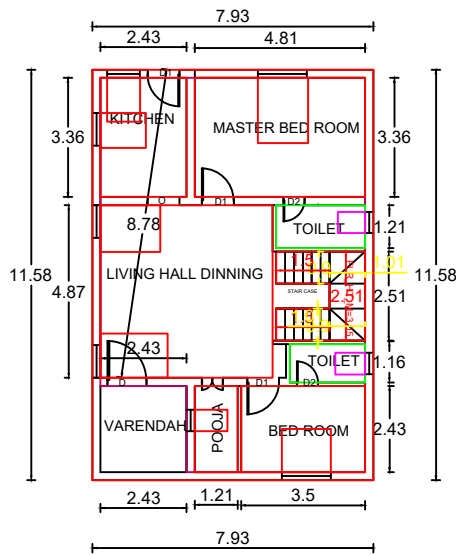
GROND FLOOR PLAN
