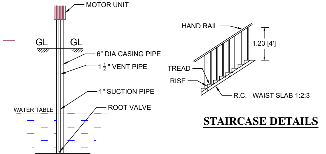
SEC.OF BOREWELL
