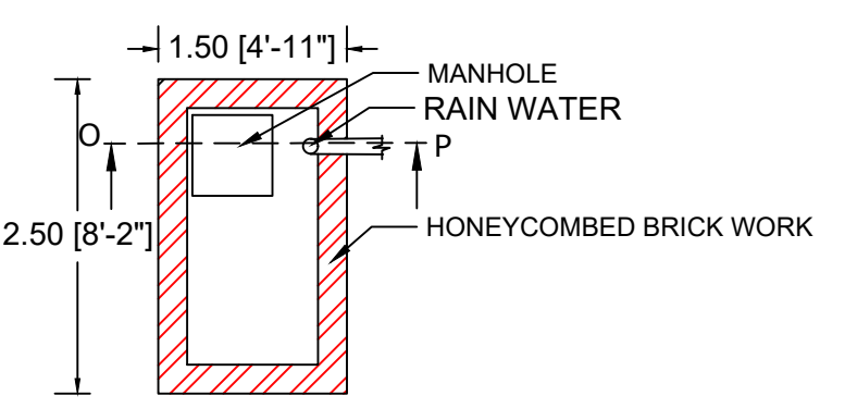
PLAN RAIN WATER HARVESTING
