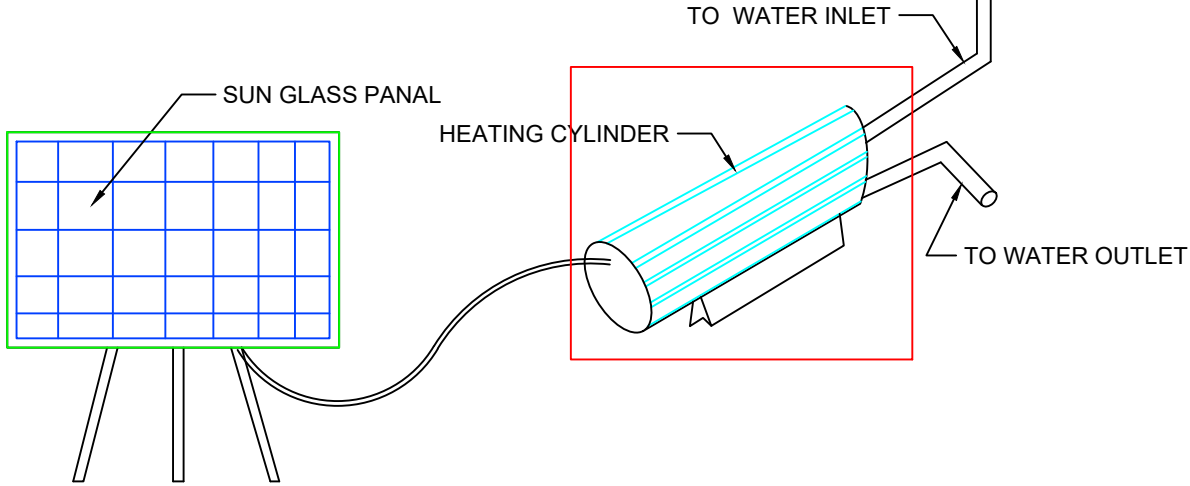
SOLAR WATER HEATING SYESTEM SCALE - N.T.S
