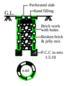
PERCOLATION PIT (NOT FOR SCALE)
