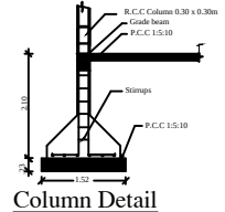
Column Detail
