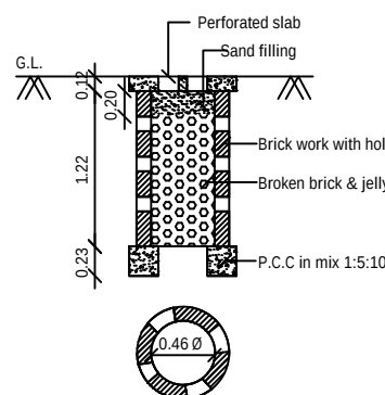
PERCOLATION PIT FOR 30 Sq. m. (Scale:- 1:50)
