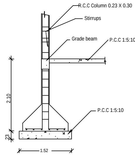
COLUMN DETAIL
