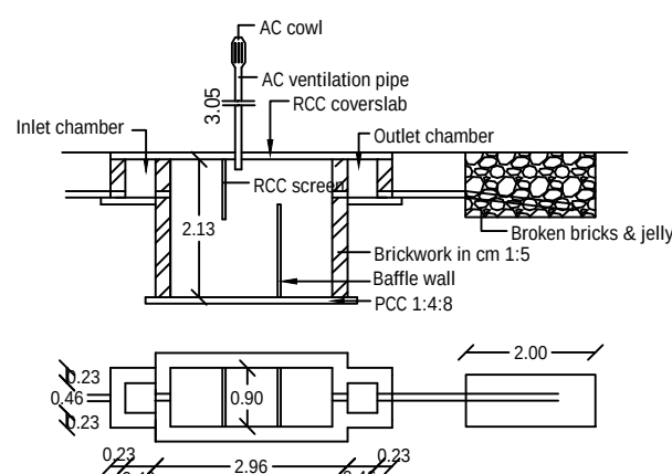
SEPTICTANK DETAILS
