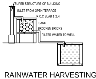
RAINWATER HARVESTING
