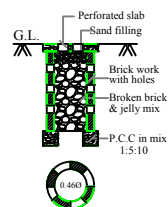
PERCOLATION PIT (NOT FOR SCALE)
