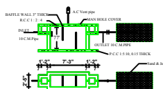
Septic tank and trench
