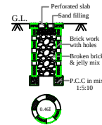
PERCOLATION PIT (NOT FOR SCALE)
