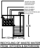
RECYCLING OF WASTE WATER FROM KITCHEN & BATHROOM
