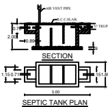
SEPTIC TANK PLAN
