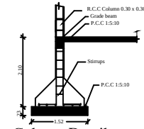
Column Detail
