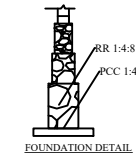
FOUNDATION DETAILS
