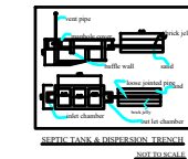
SEPTIC TANK & ABSORPTION TANK
