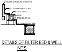
RAIN WATER HARVESTING NTS
