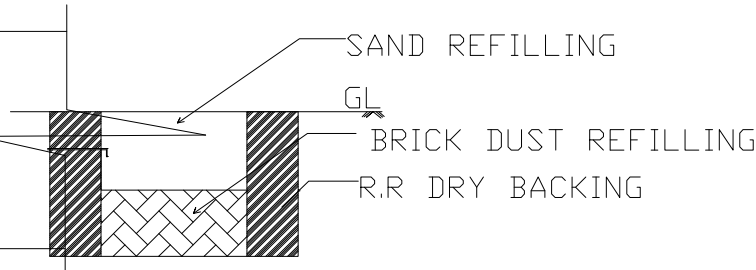
DETAILS OF RAIN WATER HARVESTING
