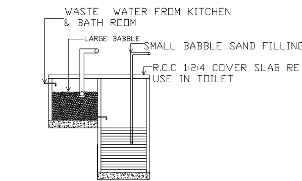
RECYCLING OF WASTE WATER FROM KITCHEN & BATHROOM
