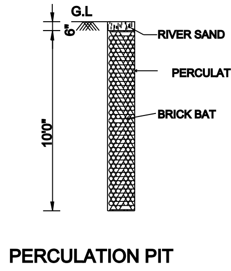
PERCULATION PIT
