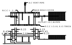
SEPTIC
