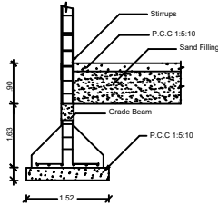
COLUMN DETAIL
