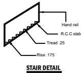
STAIR DETAIL
