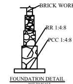
BRICK WORK
