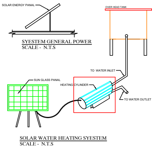
SOLAR WATER HEATING SYSTEM SCALE - N.T.S
