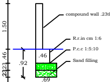
Compound wall detail
