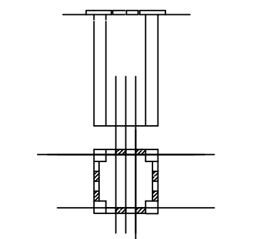
PLAN & SECTION OF RAIN WATER COLLECTION WELL
