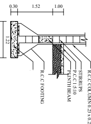
COLUMN DETAILS
