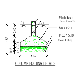
COLUMN FOOTING DETAILS
