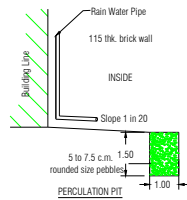
PERCOLATION PIT
