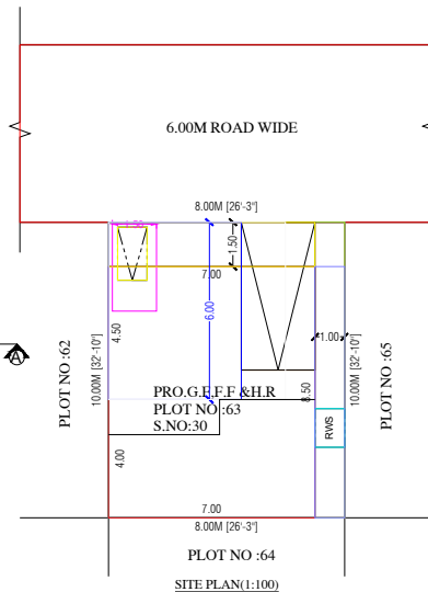
SITE PLAN(1:100)
