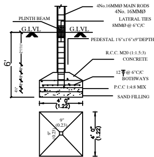
FOUNDATION DETAIL [SCALE: 1:50]
