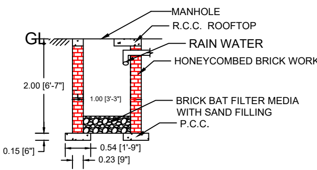
SECTION ON O - P
