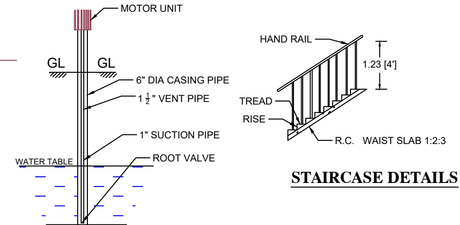
SEC.OF BOREWELL
