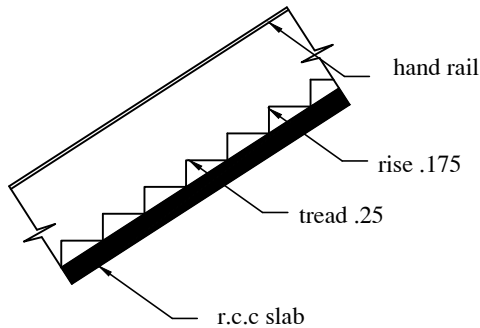
STAIR
