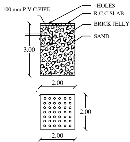
RAIN WATER COLLECTING TANK
