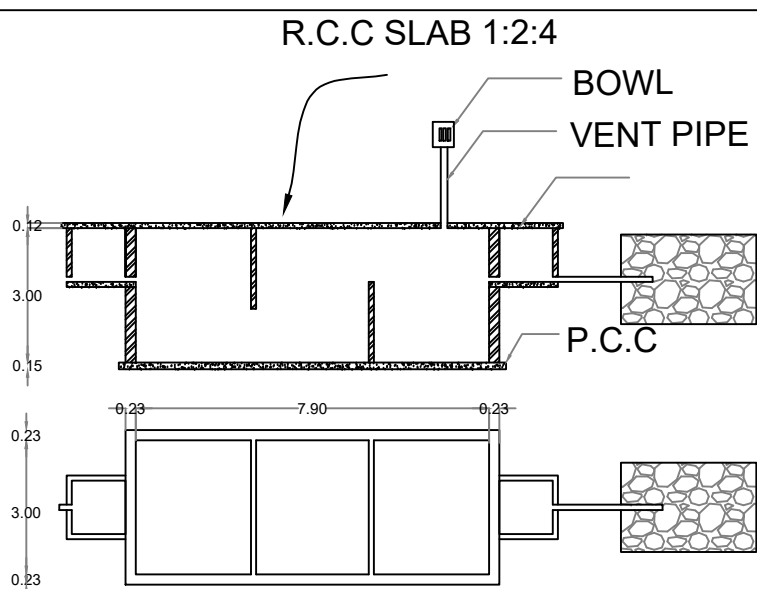
SEPTIC TANK AND TRENCH NTS
