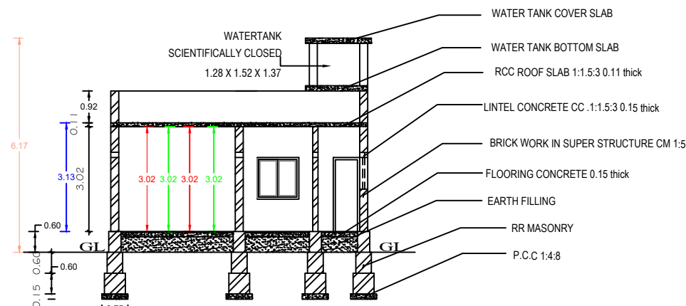
SECTION "A-B"
