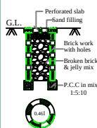
PERCOLATION PIT (NOT FOR SCALE)
