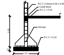
Column Detail
