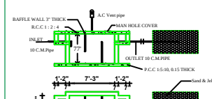
Septic tank and trench
