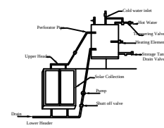
Details Of Solar Water Heater (NTS)
