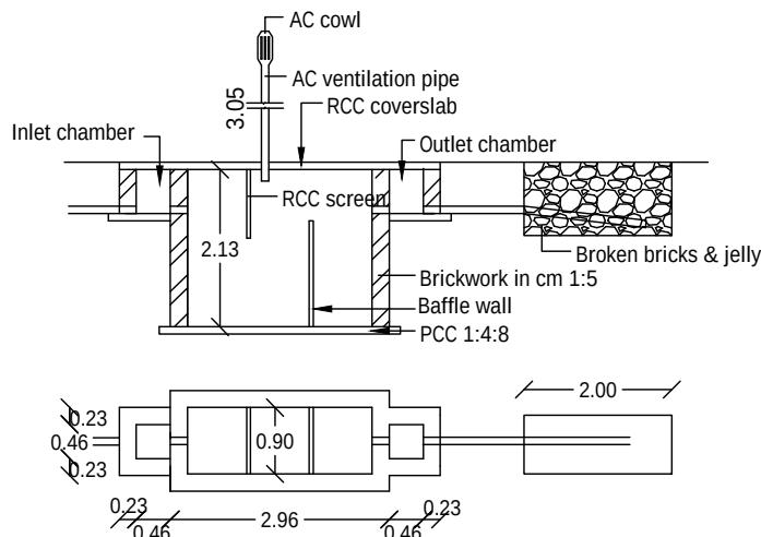
SEPTICTANK DETAILS
