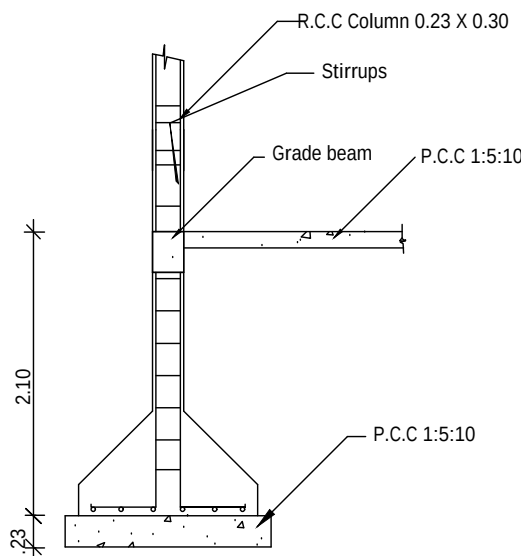
COLUMN DETAIL
