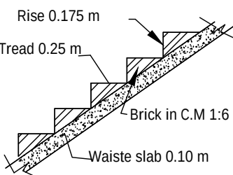
STAIR DETAILS
