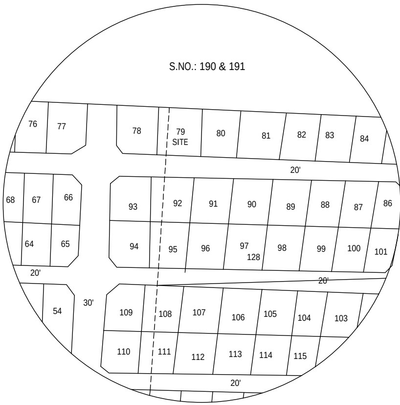
TOPO PLAN
