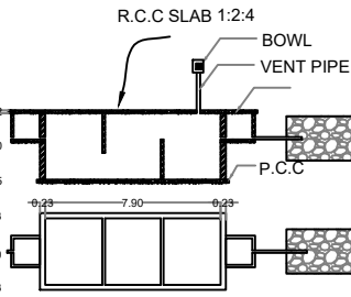
SEPTIC TANK AND TRENCH NTS
