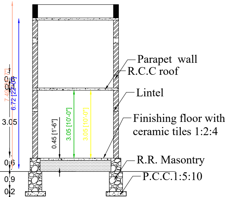
SECTION AB
