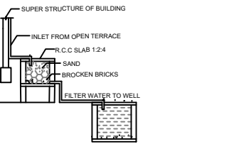
DETAILS OF FILTER BED & WELL NTS
