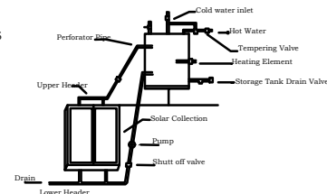
Details of Solar Water Heater (NTS)
